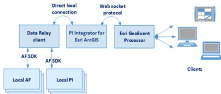
On-premises-based installation
